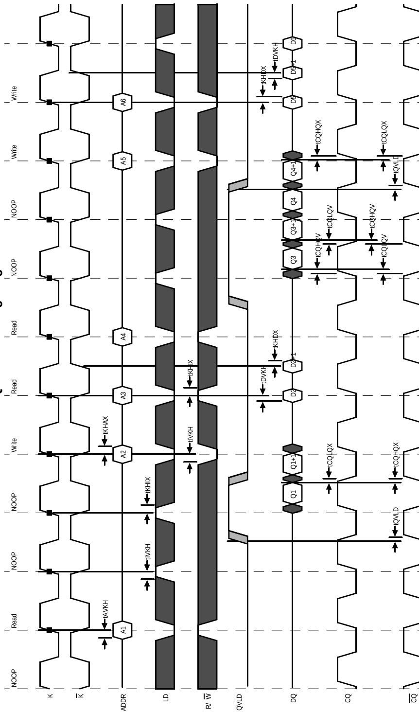
Read-Write CQ-Based Timing Diagram
