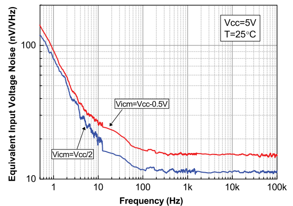
Figure 34. Noise vs. frequency at V_{CC} = 5\text{ V}
