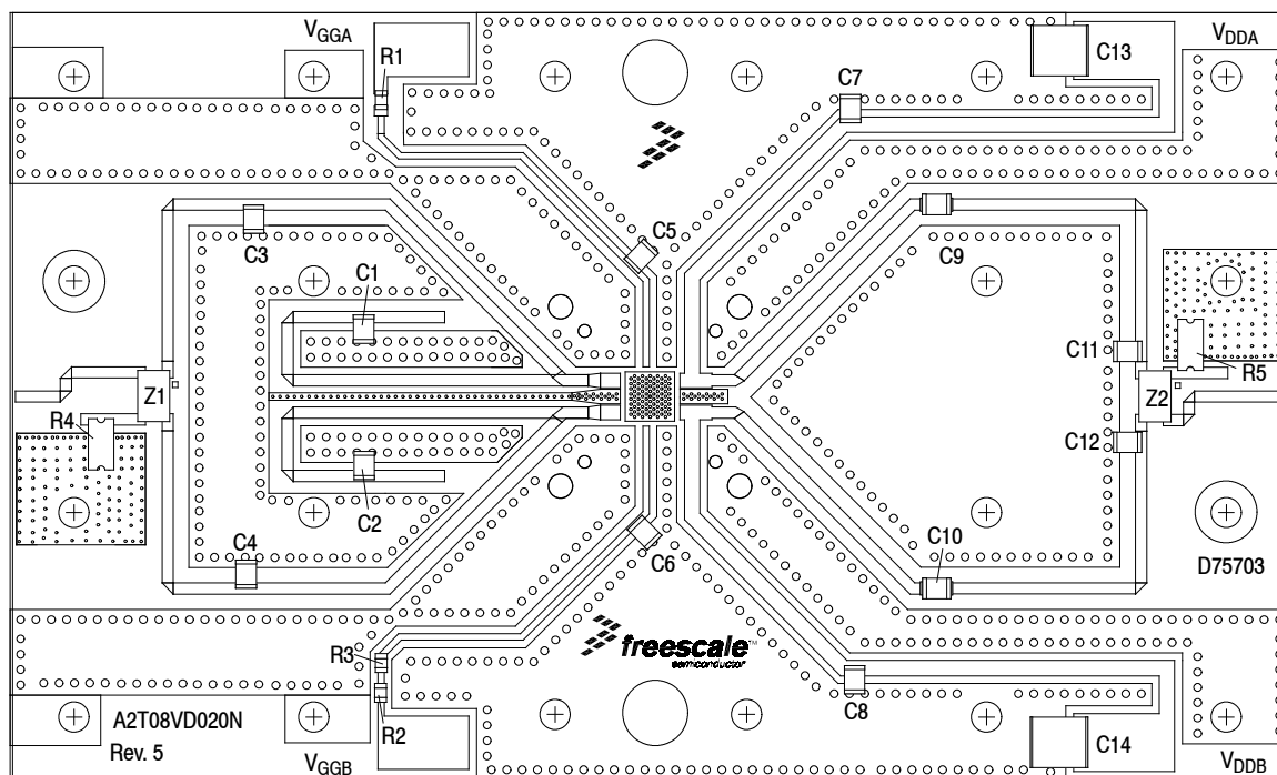
Figure 3. A2T08VD020NT1 Test Circuit Component Layout
