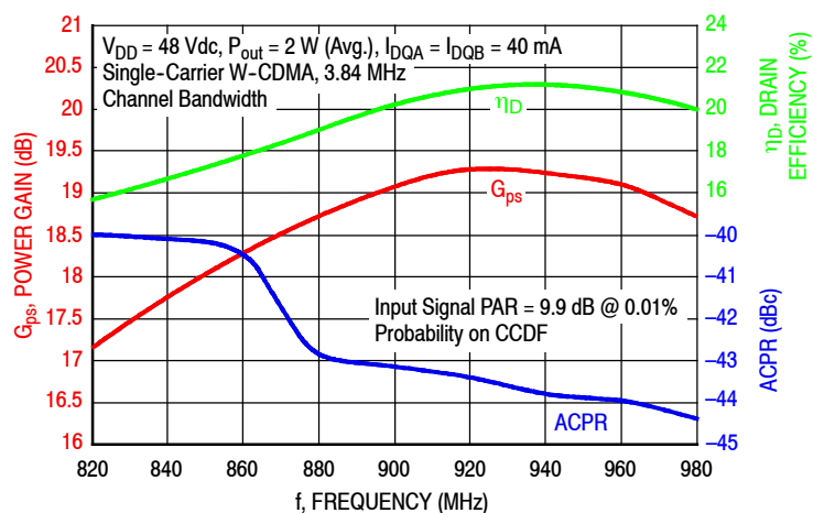
Figure 4. Broadband Performance @ P_{out} = 2 Watts Avg.
