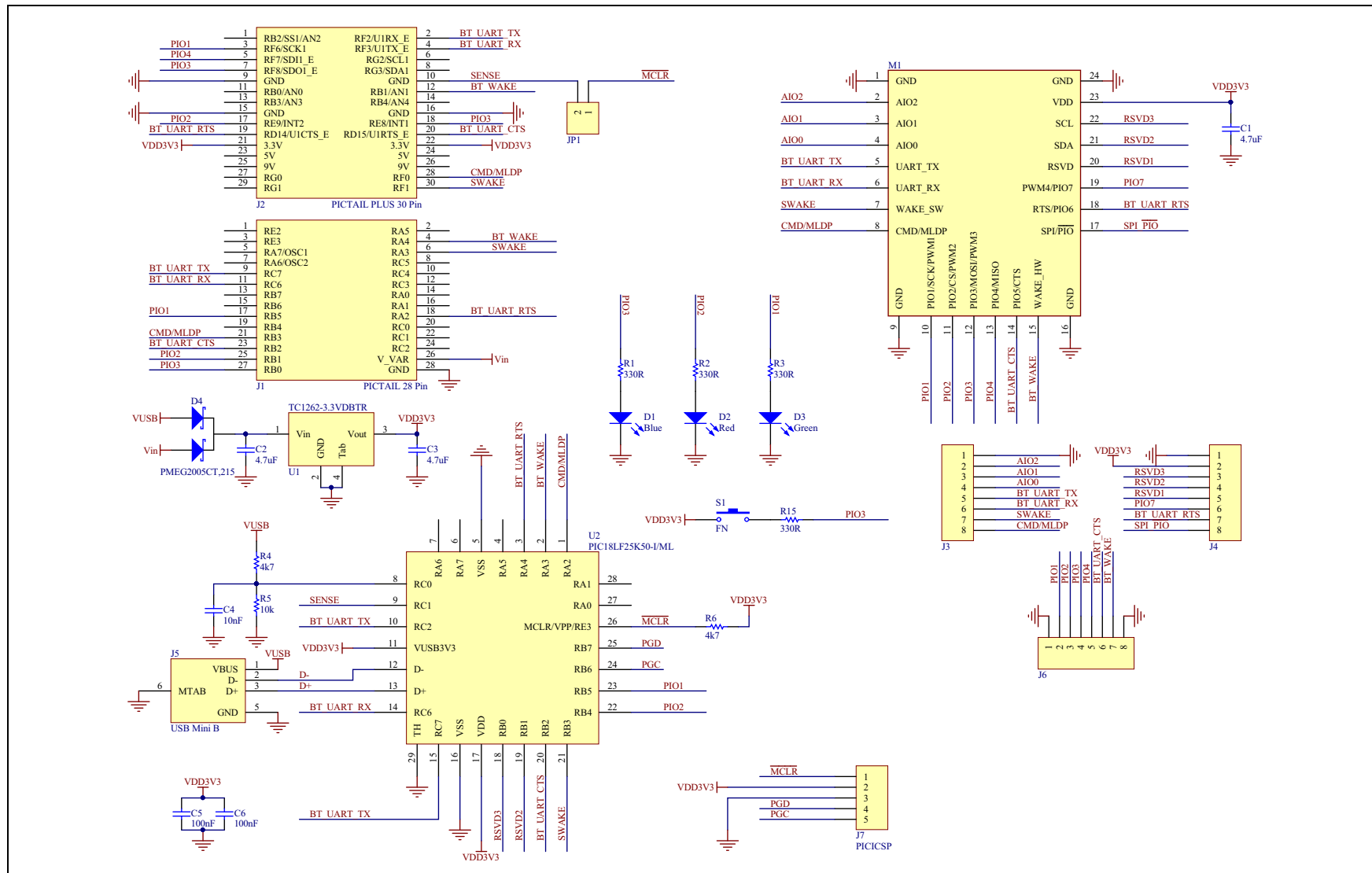
FIGURE 5-1: RN4020 TYPICAL APPLICATION SCHEMATICS
