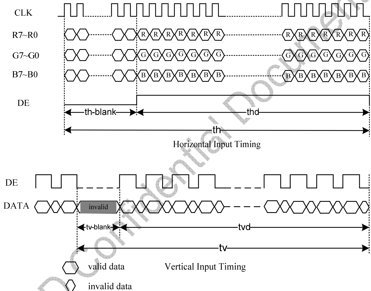
Figure 8 Timing Characteristics
