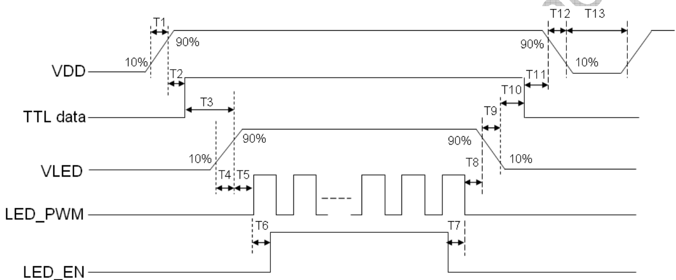
Figure 11 Power Sequence
