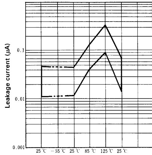
35 V/6.8 μF D case
