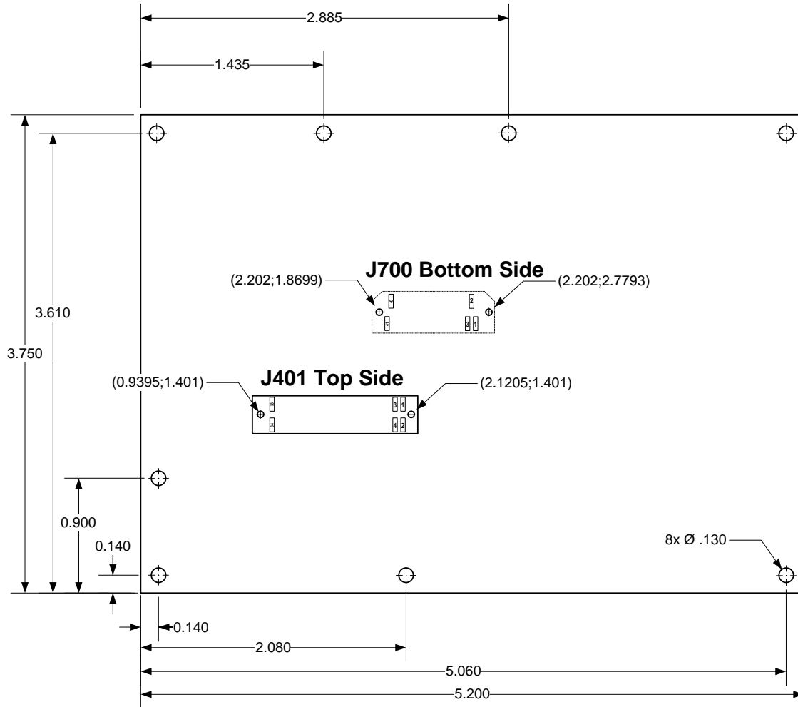
Figure 8: MityARM-335x Development Kit Outline, Mounting Hole Locations, Hirose DF9-41P-1V(32) expansion header J700 and Molex 87832-3420 LCD header J401 (Top View, inches)
