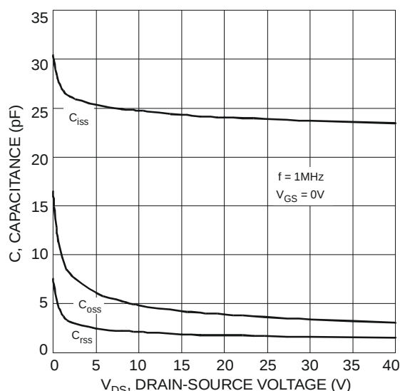
Fig. 6 Typical Capacitance
