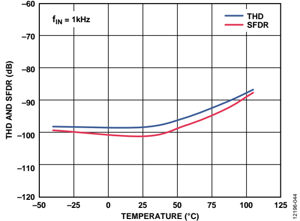
Figure 18. AD7403-8 THD and SFDR vs. Temperature
