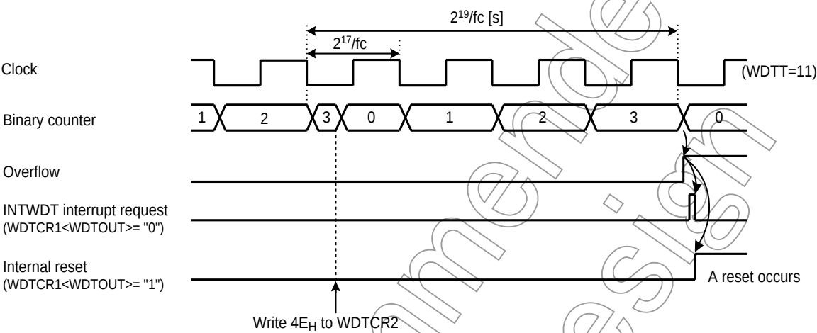
Figure 7-2 Watchdog Timer Interrupt
