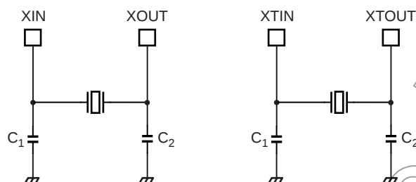
(1) High-frequency oscillation
