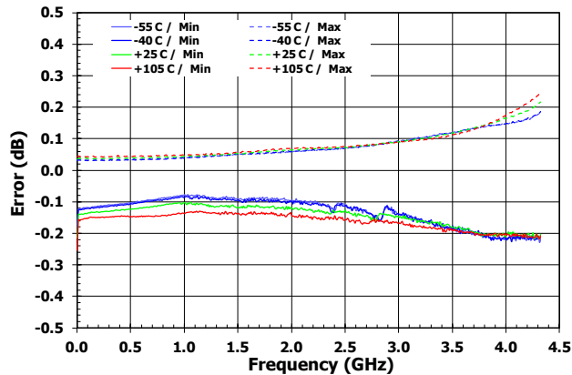
Worst Case Step Accuracy vs Frequency
