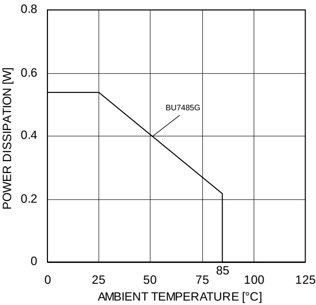
Figure 2. Derating curve
