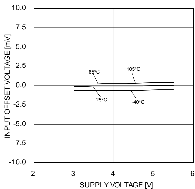
Figure 14. Input Offset Voltage – Supply Voltage ( V_{cm}=V_{DD}-1.4V , OUT=1.5V )
