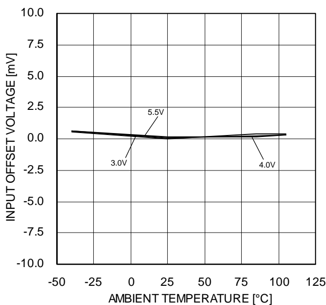
Figure 15. Input Offset Voltage – Ambient Temperature ( V_{cm}=V_{DD}-1.4V , OUT=1.5V )
