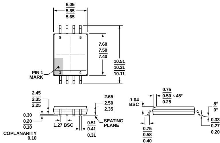
Figure 32. 8-Lead Standard Small Outline Package, with Increased Creepage [SOIC_IC] Wide Body (RI-8-1) Dimensions shown in millimeters
