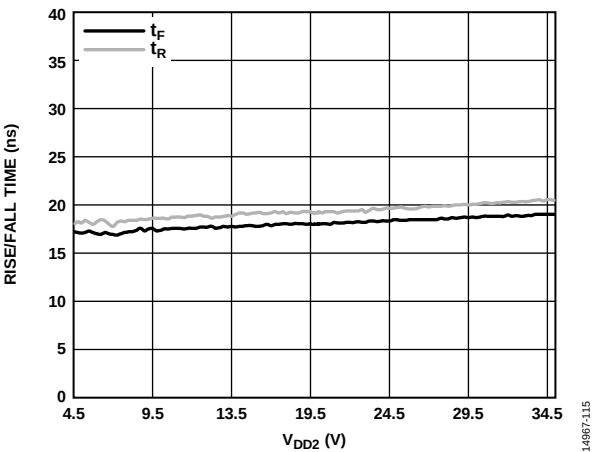
Figure 16. Rise and Fall Time vs. V_{DD2} , 2 nF Load, 3.9 \Omega Resistor
