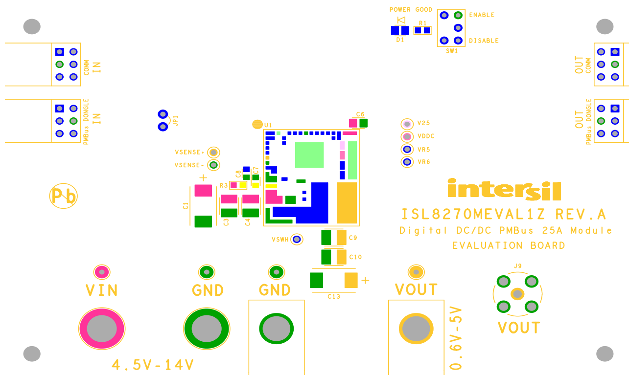
FIGURE 9. PCB - TOP SILK SCREEN
