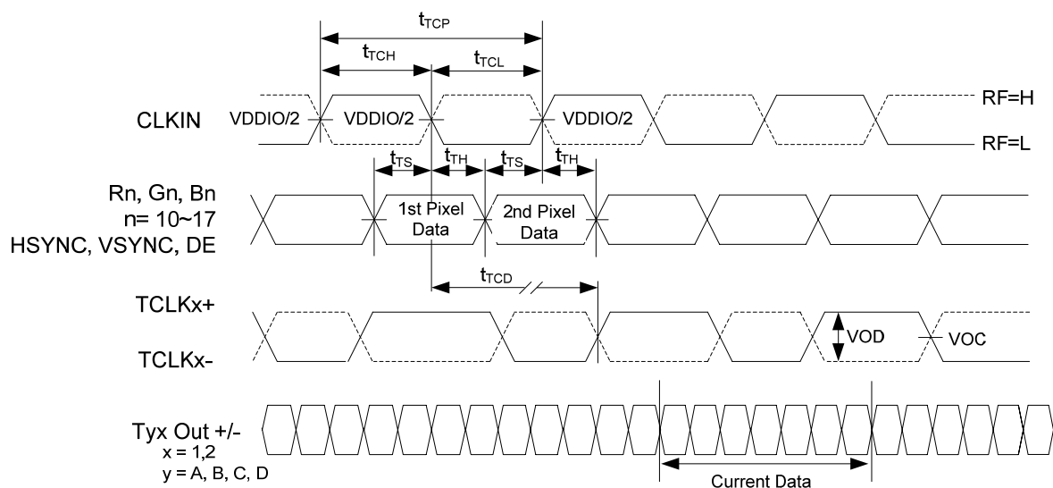
Figure 5. LVCMOS Input AC Timing Diagrams (DDR function ON)
