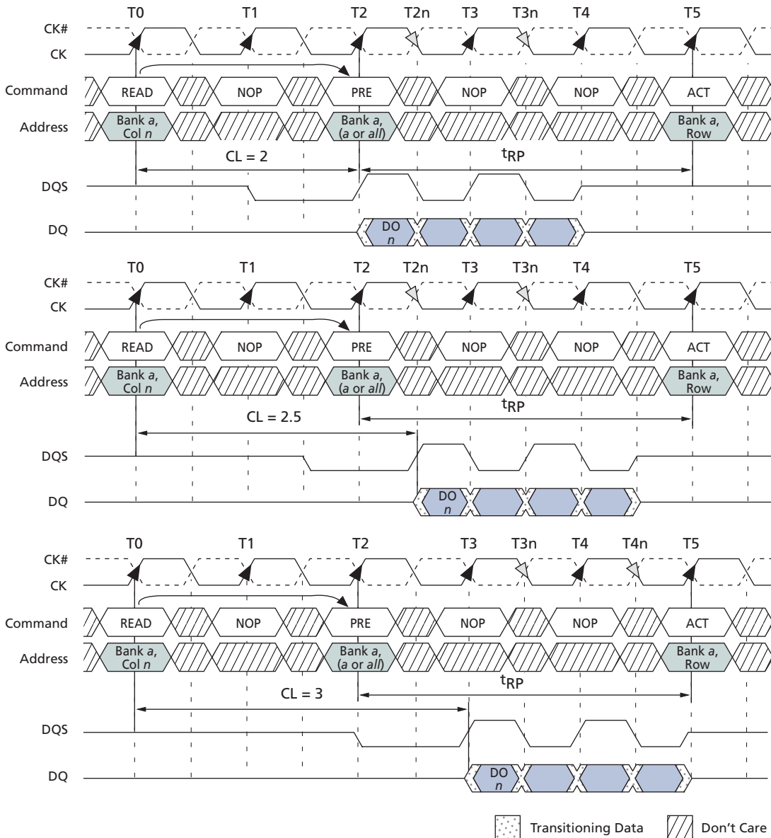
Figure 32: READ-to-PRECHARGE
