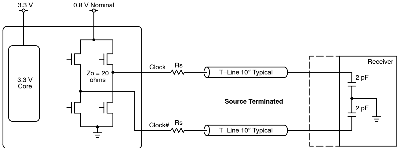
Figure 16. NMOS Push-Pull Buffer Diagram
