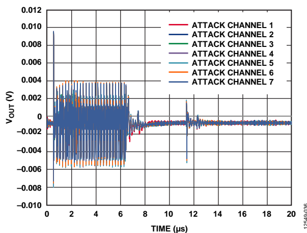
Figure 34. DAC-to-DAC Crosstalk
