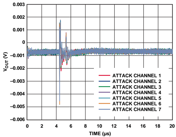
Figure 33. Analog Crosstalk
