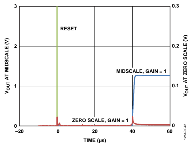
Figure 40. Hardware Reset
