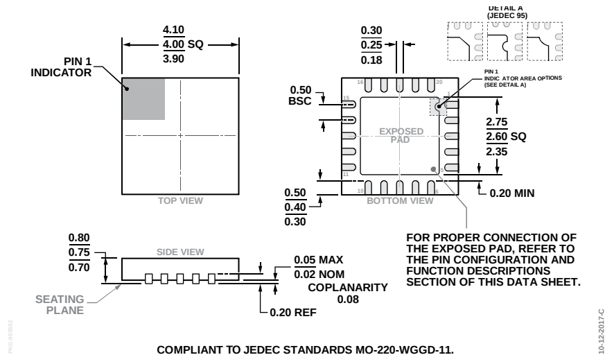
COMPLIANT TO JEDEC STANDARDS MO-220-WGGD-11. Figure 54. 20-Lead Lead Frame Chip Scale Package [LFCSP] 4 mm × 4 mm Body and 0.75 mm Package Height (CP-20-8) Dimensions shown in millimeters
