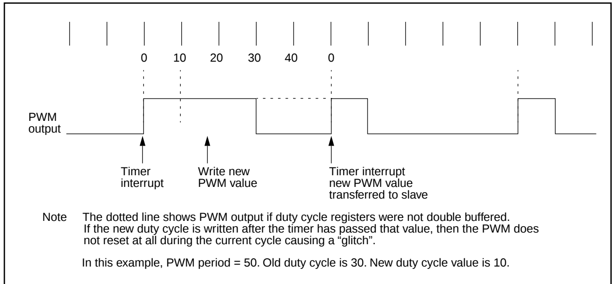
FIGURE 12-6: PWM OUTPUT
