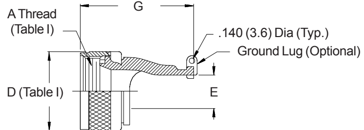
450ES002 STRAIGHT ROTATABLE COUPLING
