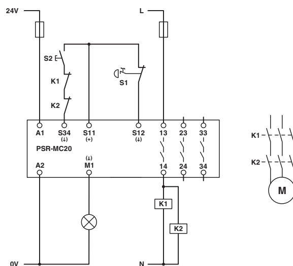
Figure 13 Emergency stop monitoring/manual, monitored start
