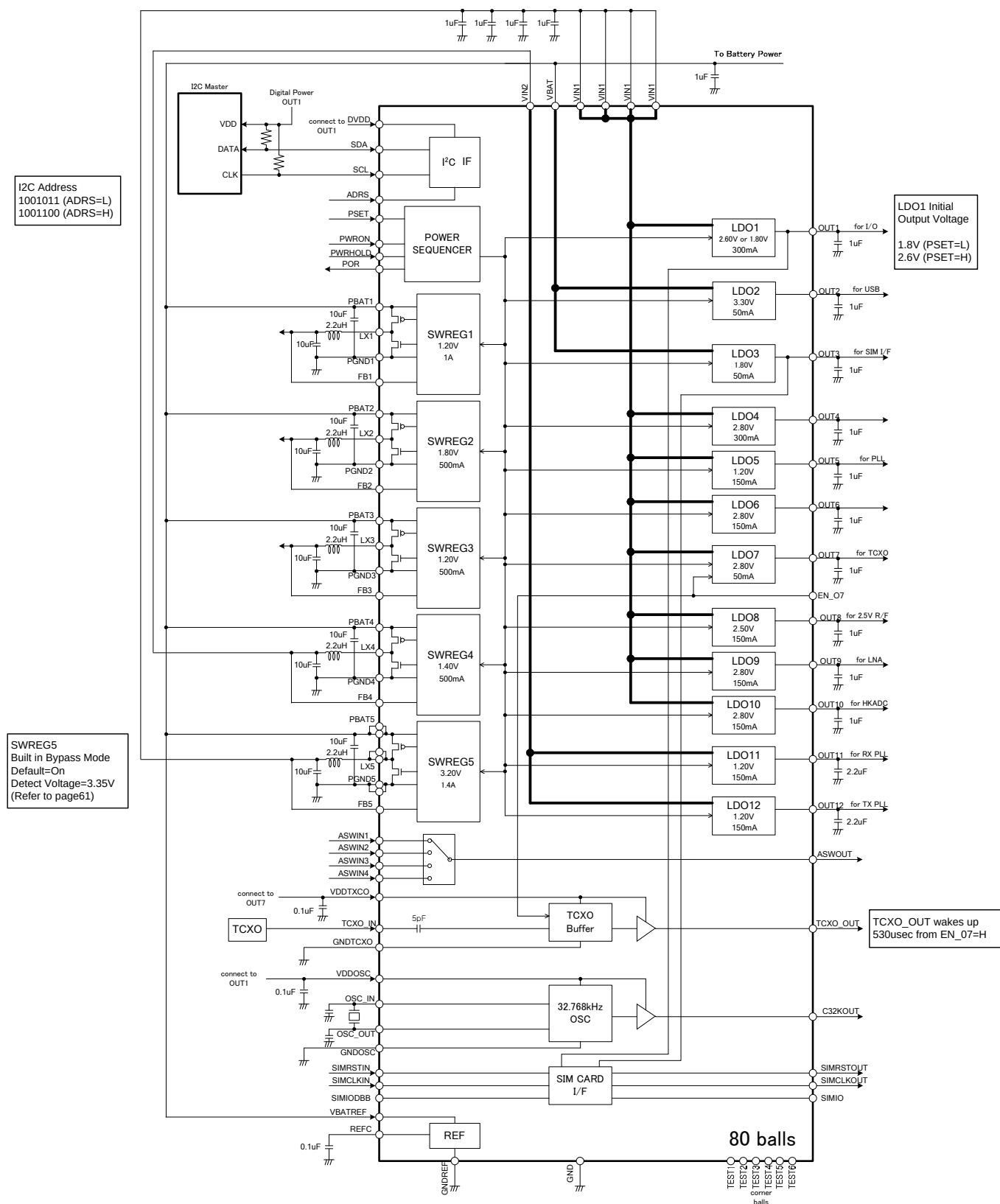
Figure 1. Block Diagram
