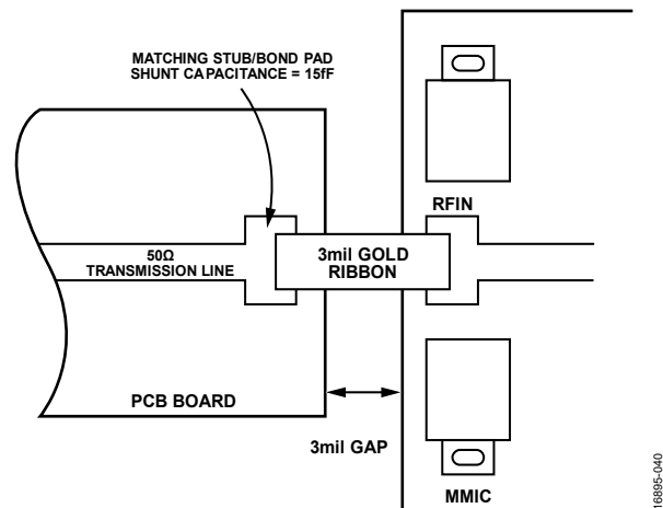
Figure 41. High Frequency Input Wideband Matching
