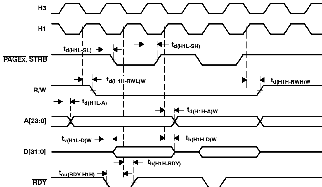
Figure 21. Timing for Memory ( \text{STRB} = 0 and \overline{\text{PAGEX}} = 0 ) Write
