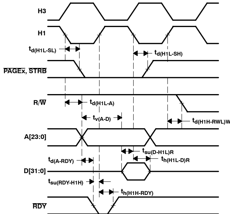
Figure 20. Timing for Memory ( \text{STRB} = 0 and \overline{\text{PAGEX}} = 0 ) Read
