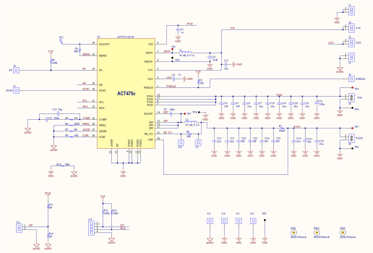
Figure 4. Schematic
