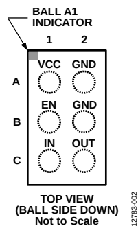
Figure 2. Pin Configuration
