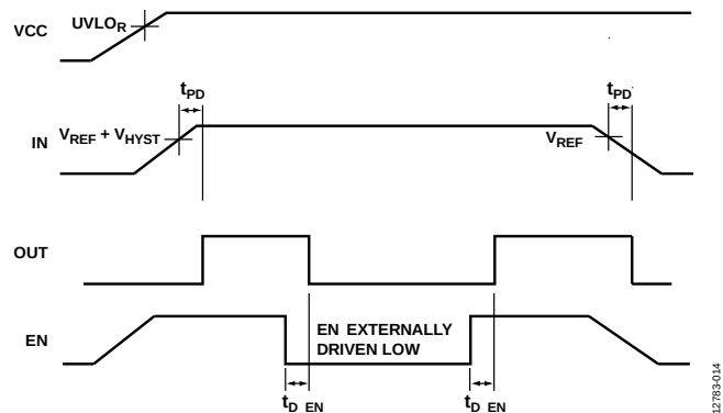
Figure 14. Timing Diagram
