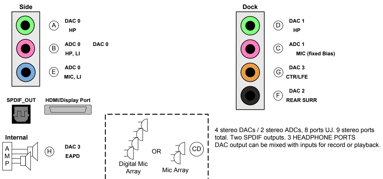
Figure 13. Port Configurations
