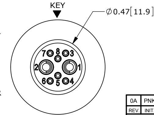
WIRING END ASSY: W7A82-8SG-300 SHOWN
