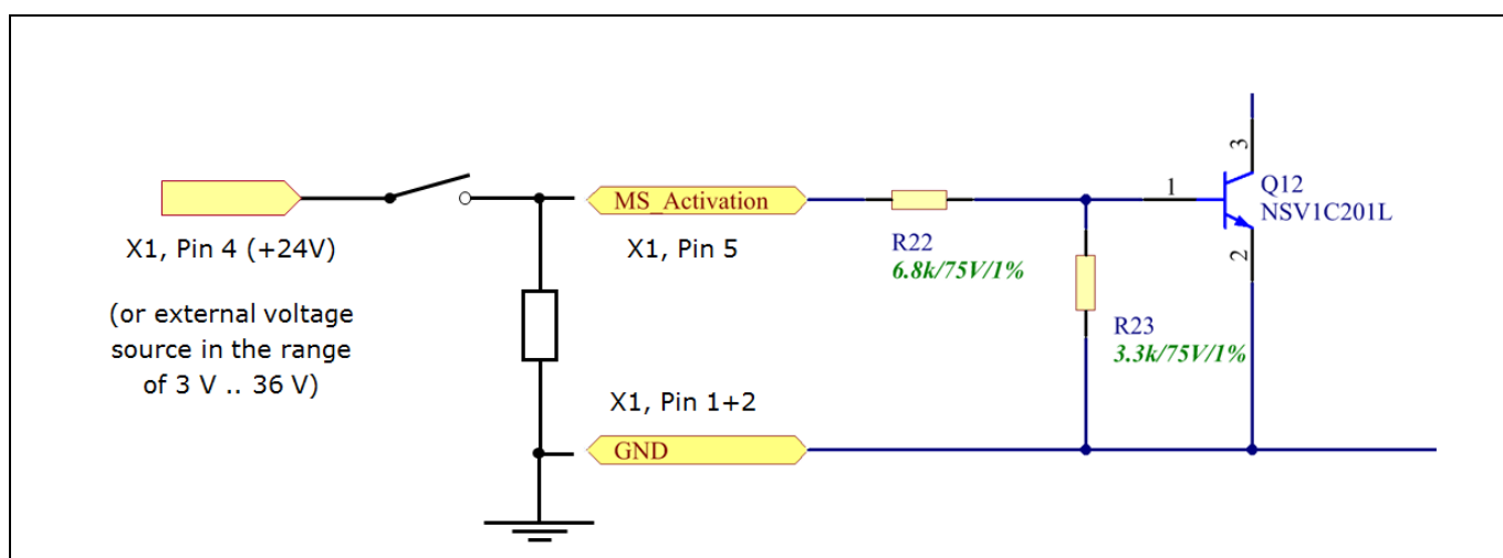
Figure 8 Input Stage
