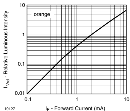
Figure 1. Relative Luminous Intensity vs. Forward Current
