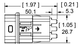
Short Depth - For Solder Termination to PCB
