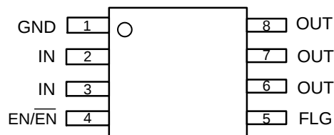
MSOP-8
