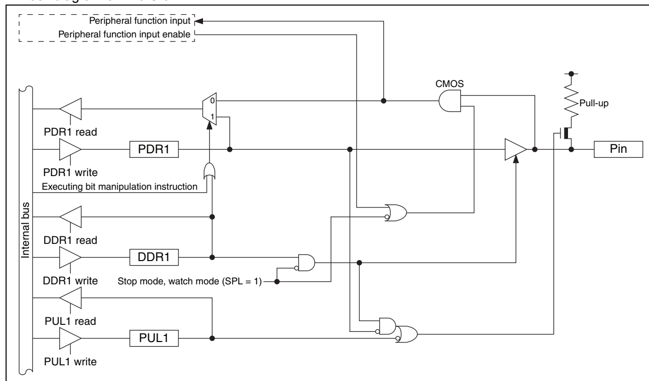
• Block diagram of P10/UI0
