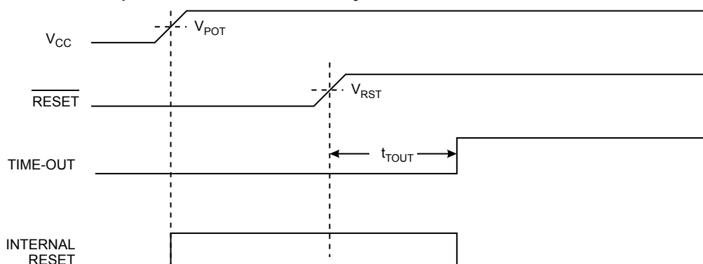
Figure 15-3. MCU Start-up, \overline{\text{RESET}} Extended Externally
