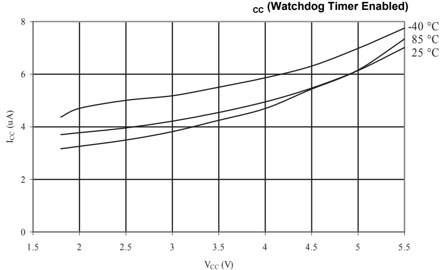
Figure 34-106. ATmega168A: Power-Down Supply Current vs. V_{CC} (Watchdog Timer Enabled)
