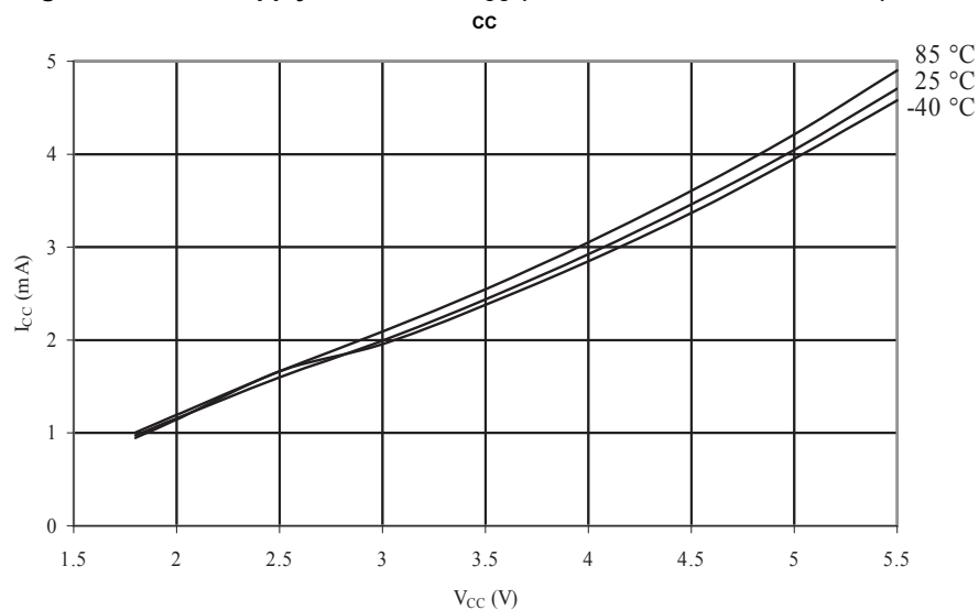
Figure 34-5. ATmega48A: Active Supply Current vs. V_{CC} (Internal RC Oscillator, 8MHz)
