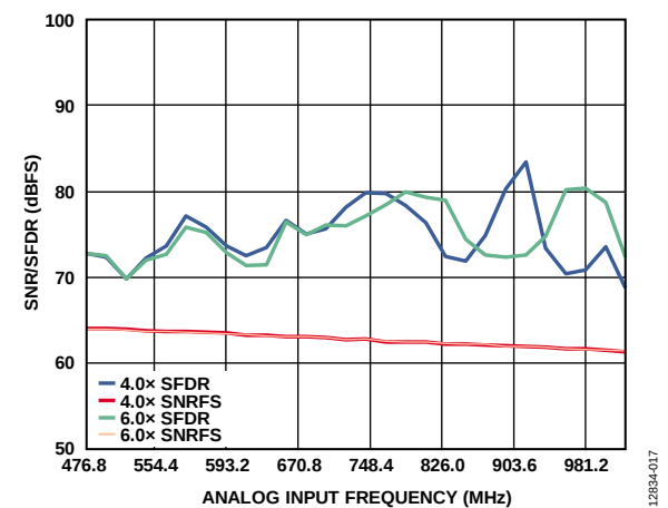
Figure 17. SNR/SFDR vs. Analog Input Frequency ( f_{IN} ); 500 MHz < f_{IN} < 1 GHz; Buffer Control1 (0x018) = 4.0x and 6.0x
