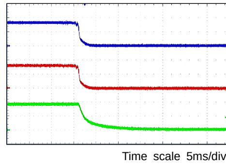
Figure 20. Power-down EN = V_{IN} V_{IN} = 3.3V , V_O = 1.8V , I_O = 0A
