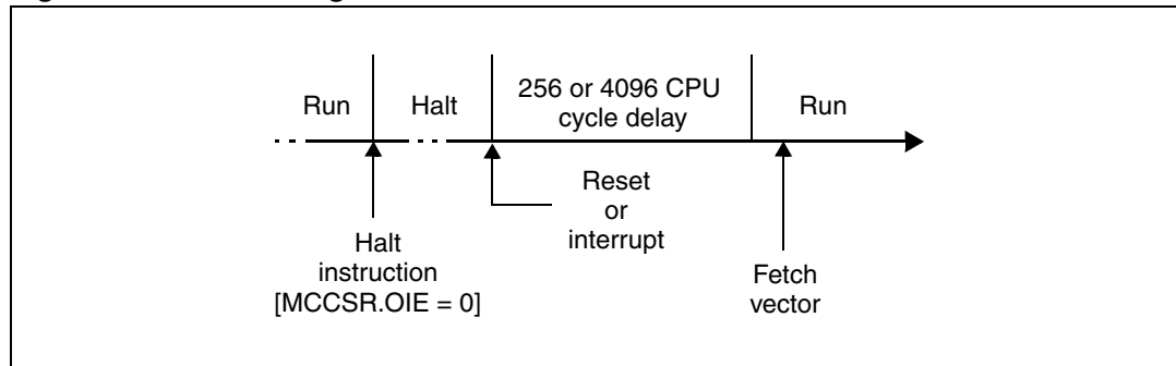
Figure 26. HALT timing overview
