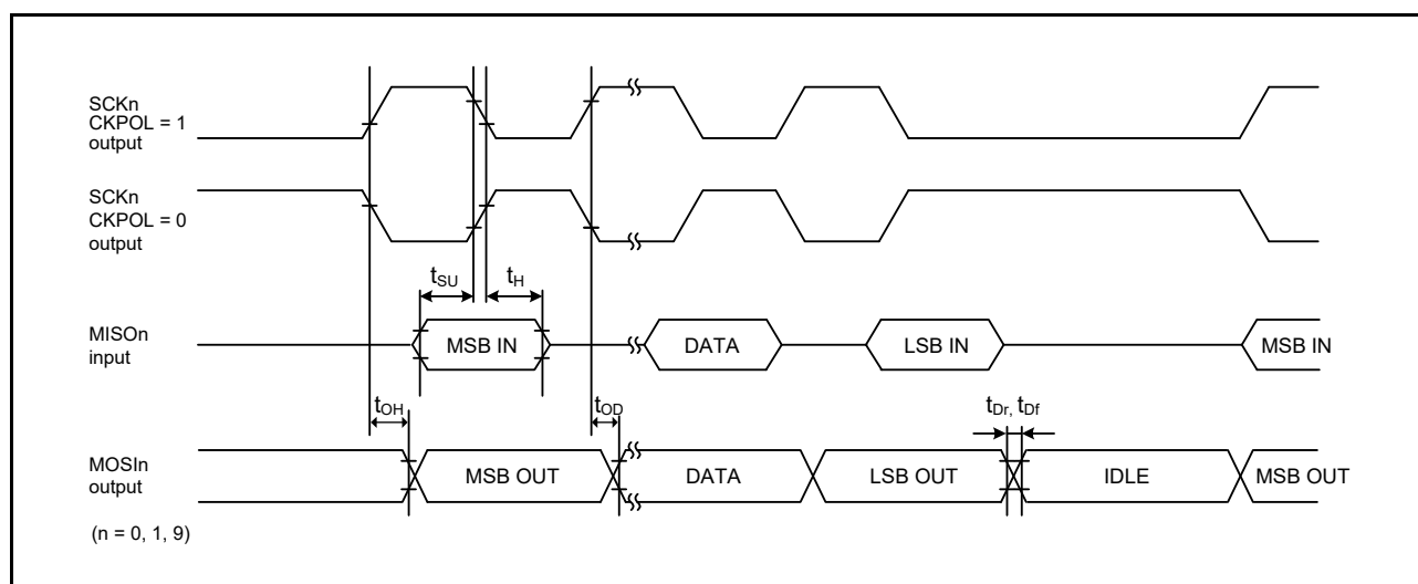
Figure 2.45 SCl simple SPI mode timing (master, CKPH = 0)
