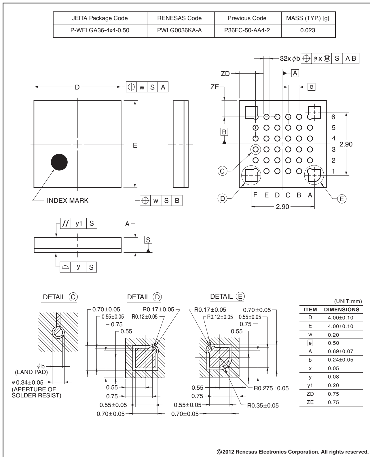
Figure 1.4 LGA 36-pin
