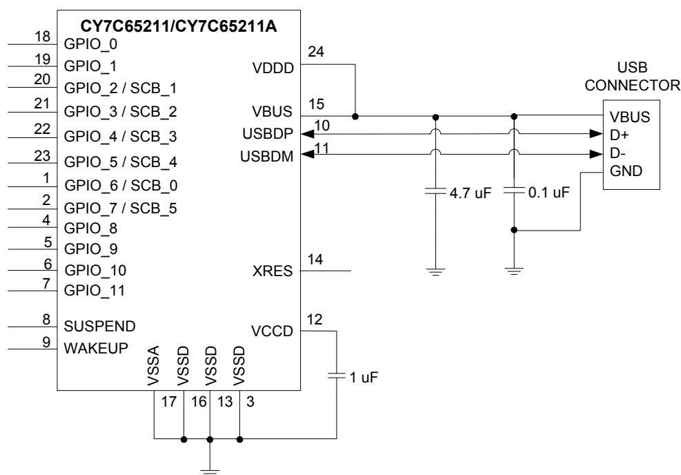
Figure 3. Bus-Powered Configuration
