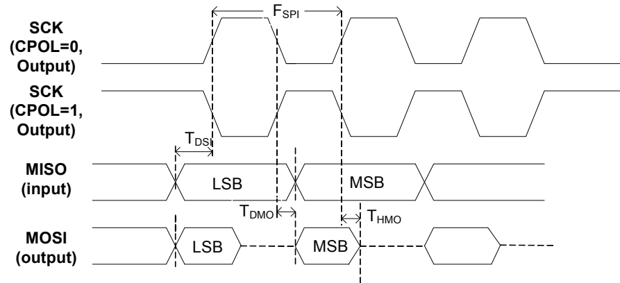
Figure 1. SPI Master Timing
