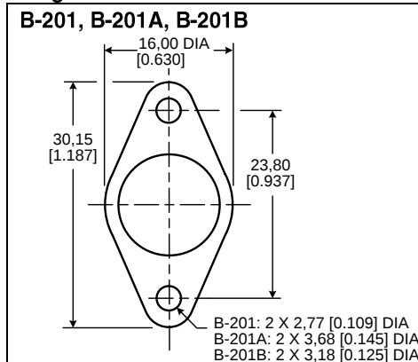
Figure 19. 3001/3004 Brackets
