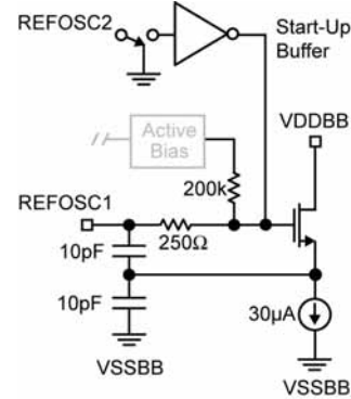
Figure 5. REFOSC Pin
