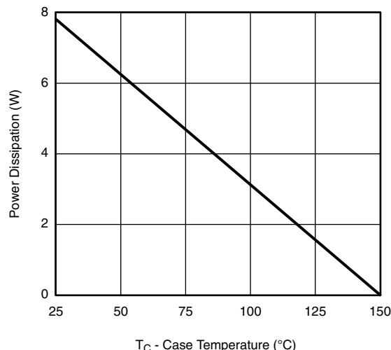
Power Derating
