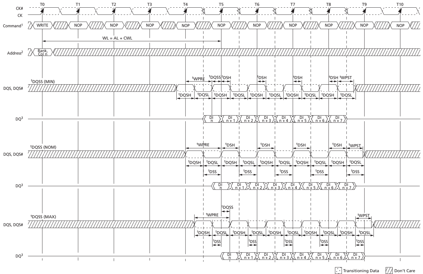
Figure 86: WRITE Burst
