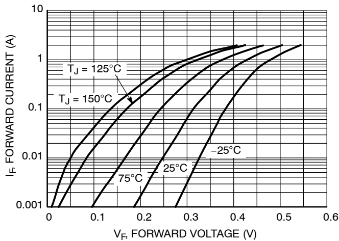
Figure 1. Forward Voltage
