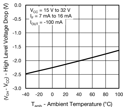
Fig. 7 - High Level Voltage Drop vs. Ambient Temperature
