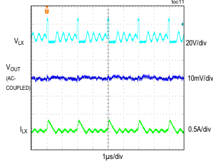
STEADY-STATE PERFORMANCE
